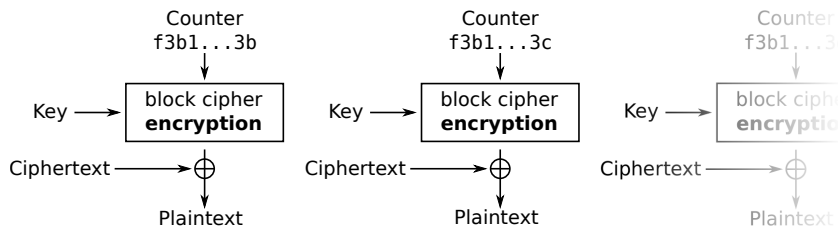
Figure 18: Counter (CTR) mode decryption
