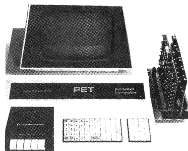
BETSI is the new Interface/Motherboard from Forethought Products—the makers of KIM1™—which allows users of Commodore's PET Personal Computer to instantly work with the scores of memory and I/O boards developed for the S-100 (Imsaï/Altair type) bus. BETSI is available from stock on a single 5½" x 10" printed circuit card.
